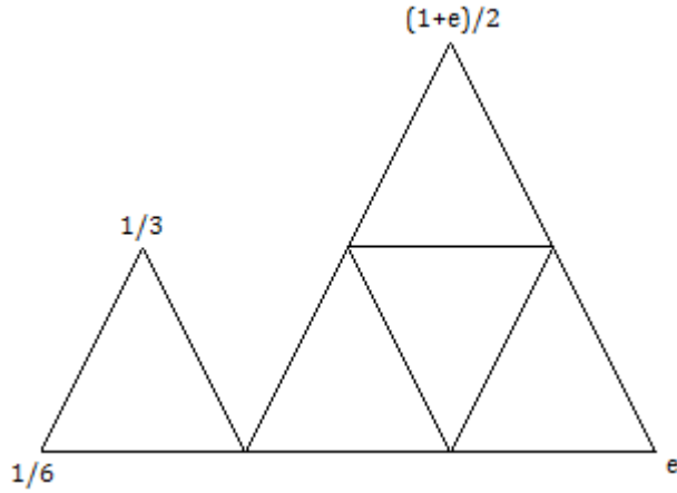
Figure 2: F_0^0
