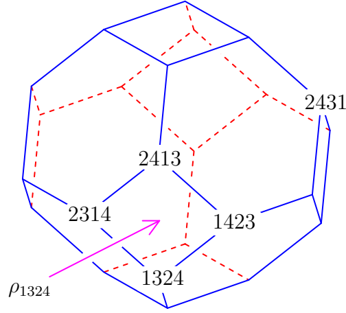
FIGURE 3. The facet \rho_{1324} of type (2, 2) and w = 2431 .
