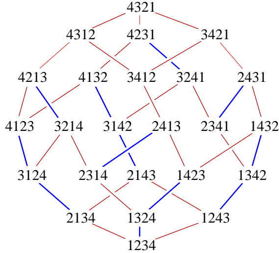
FIGURE 1. The fibers of P_i : S_4 \rightarrow S_3 \times S_2
